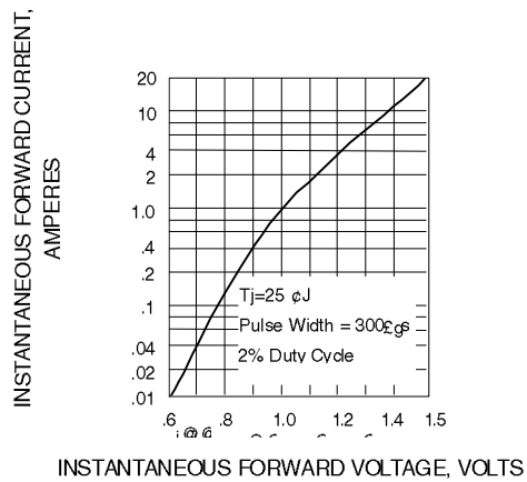
Fig. 1-TYPICAL FORWARD CHARACTERISTICS
