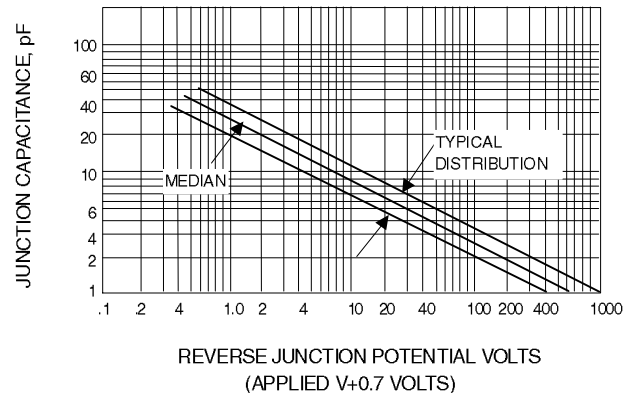
Fig. 2-JUNCTION CAPACITANCE
