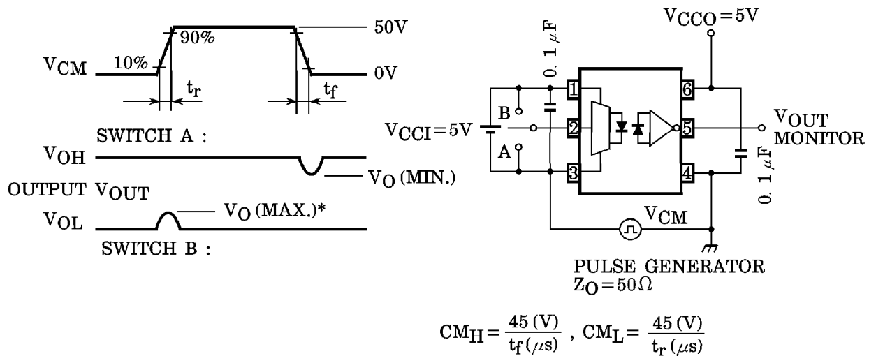
TEST CIRCUIT 4 : Common Mode Transient Immunity (TLP216)
