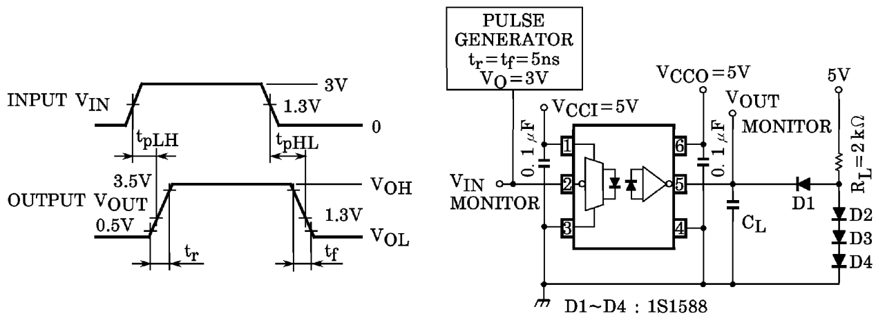
TEST CIRCUIT 1 : t_{pLH} , t_{pHL} , t_r and t_f (TLP215)
