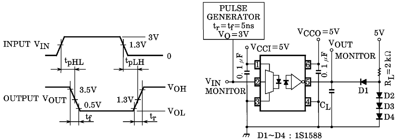
TEST CIRCUIT 3 : t_{pLH} , t_{pHL} , t_r and t_f (TLP216)
