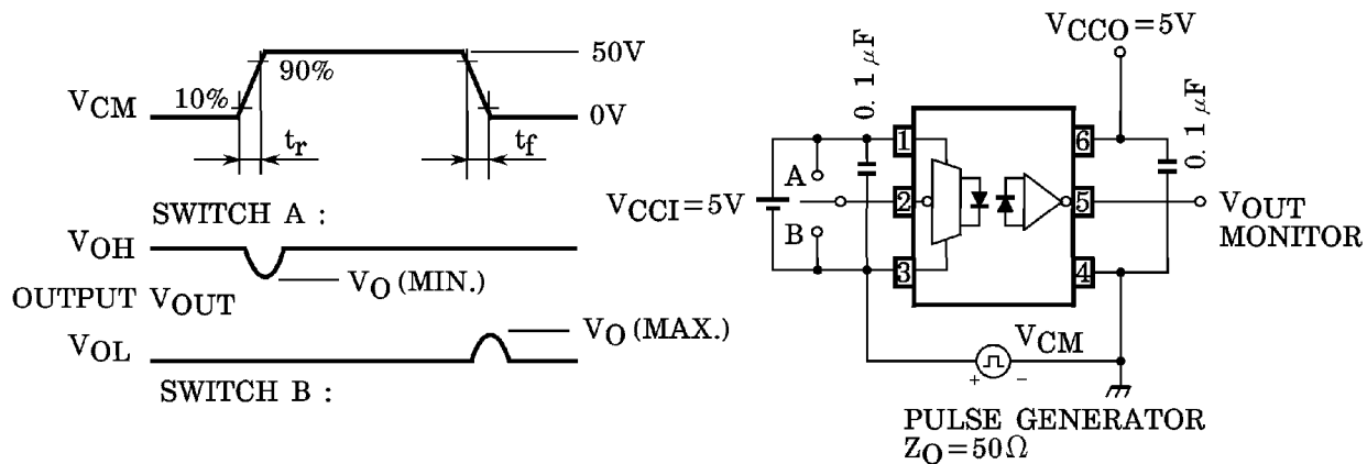
TEST CIRCUIT 2 : Common Mode Transient Immunity (TLP215)
