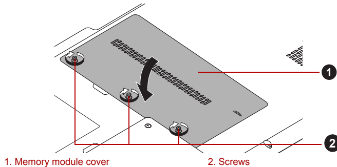
Seating the memory module cover
