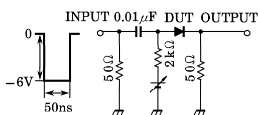
Fig.1 : REVERSE RECOVERY TIME ( t_{rr} ) TEST CIRCUIT
