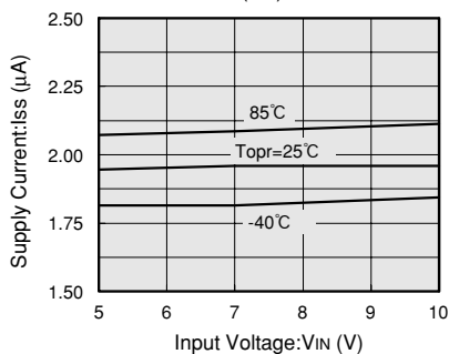
XC62FP5002 (5V)
