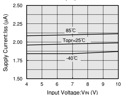
XC62FP4002 (4V)
