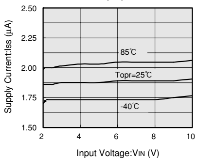
XC62FP2002 (2V)
