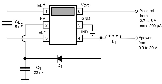
FIGURE 4: SPLIT SUPPLY APPLICATION CIRCUIT
