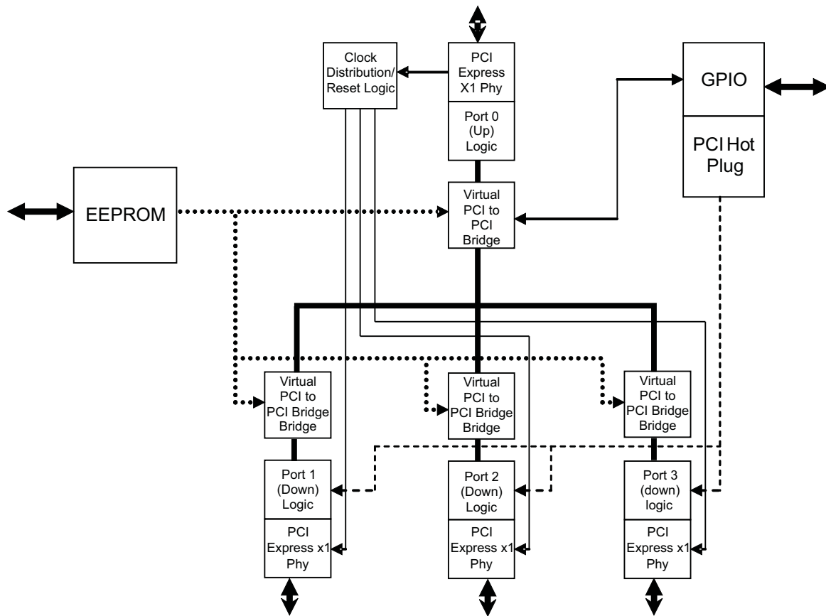
Figure 3-1. Block Diagram
