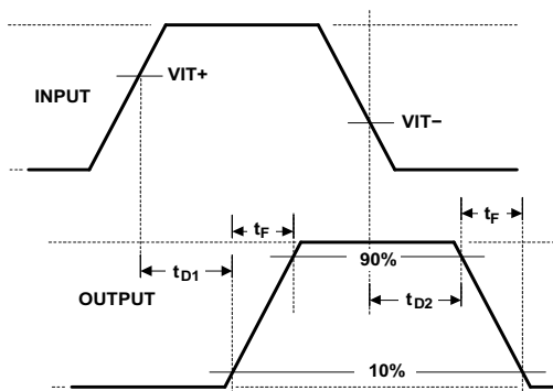
Figure 5. Timing Diagram
