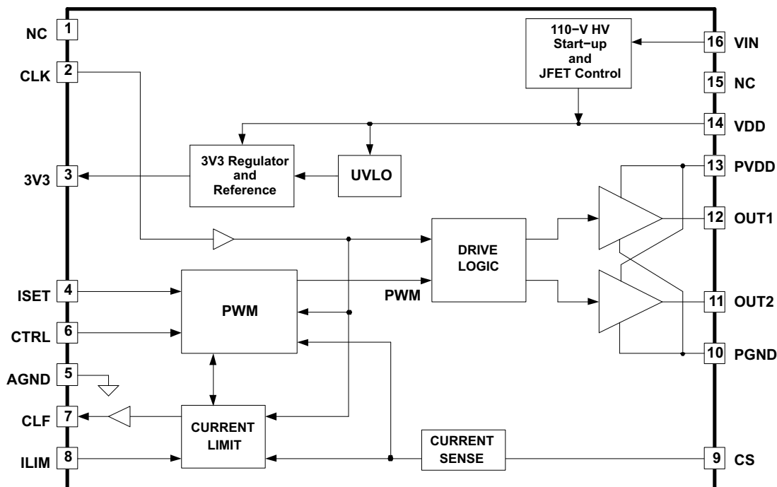
Figure 7. UCD8620
