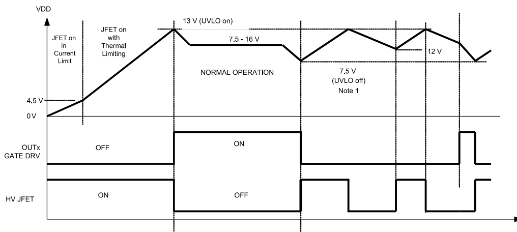
Figure 40. UCD8620 JFET Operation Waveforms
