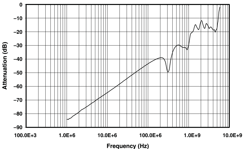
Figure 2. OFF Isolation
