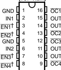
TPS2044B/TPS2054B D PACKAGE (TOP VIEW)
