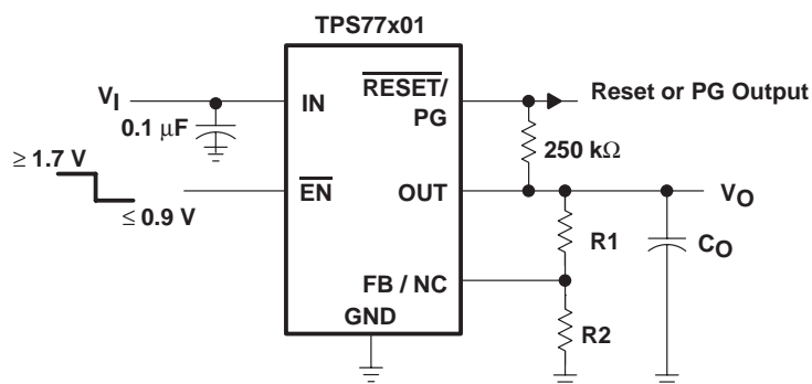
Figure 25. TPS77x01 Adjustable LDO Regulator Programming
