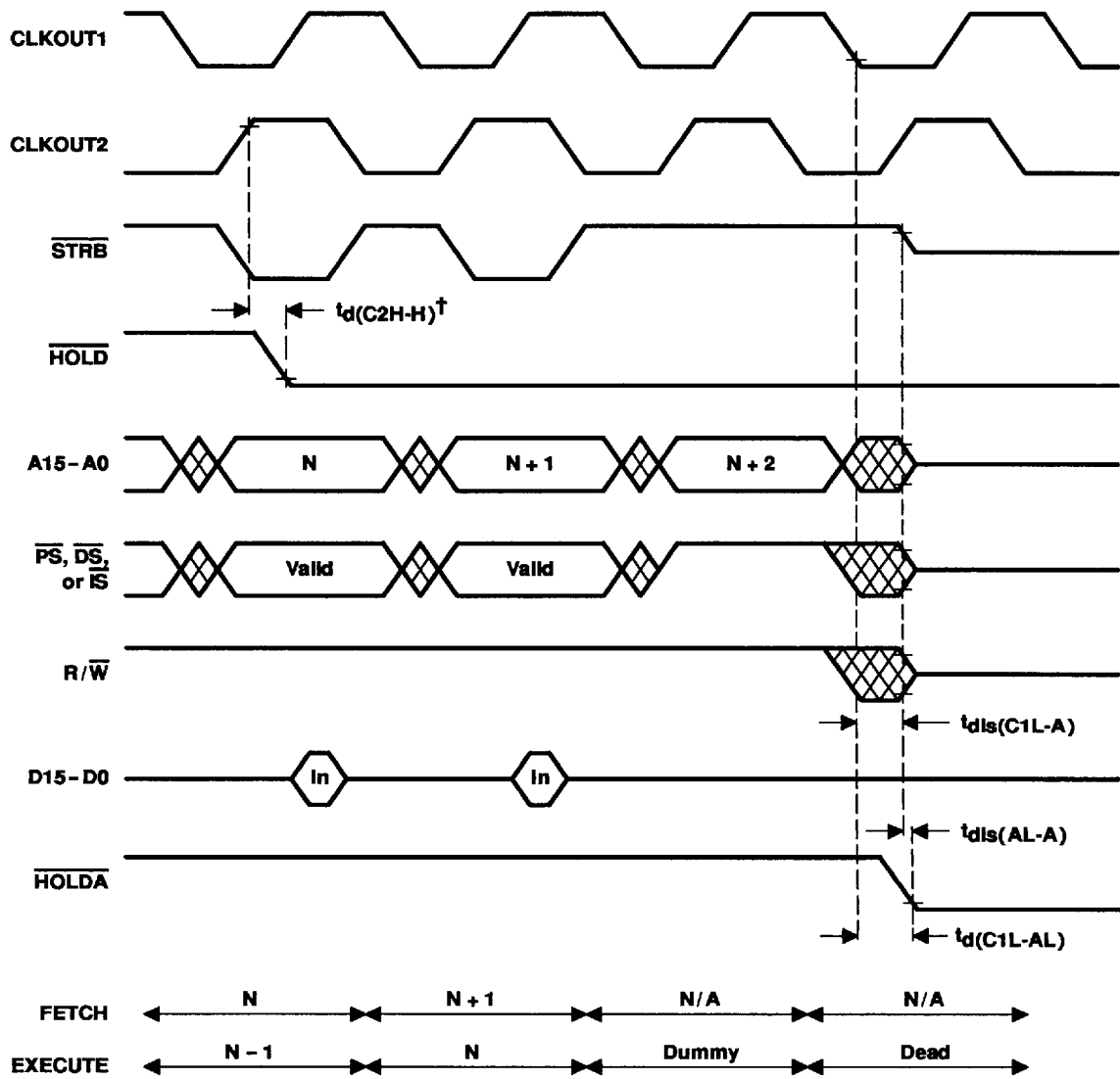
Figure 16. \overline{\text{HOLD}} Timing (Part A)
