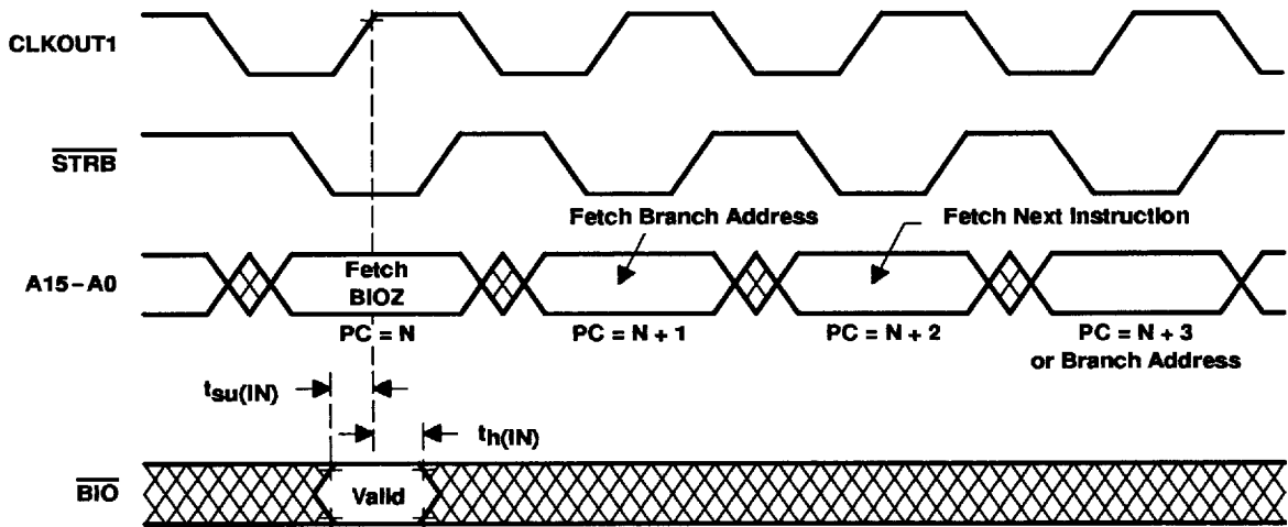
Figure 14. BIO Timing
