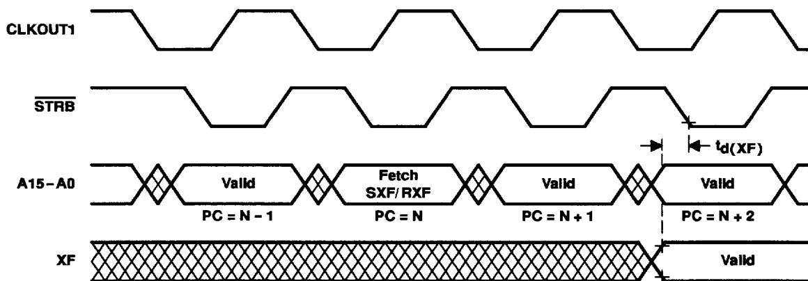
Figure 15. External Flag Timing
