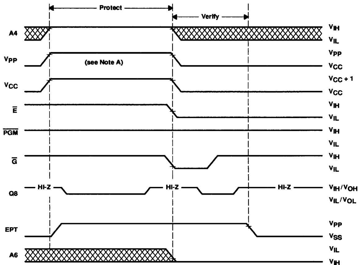
Figure 27. EPROM-Protection Timing
