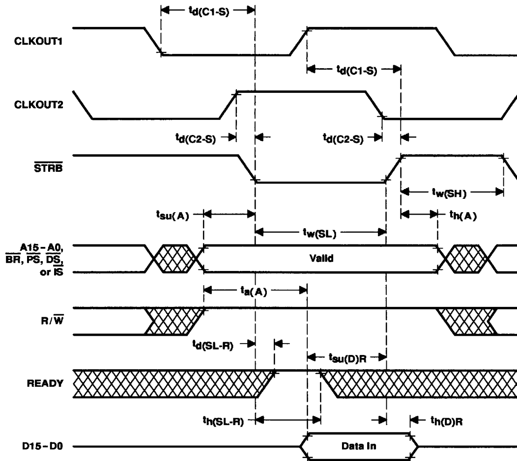
Figure 7. Memory-Read-Cycle Timing
