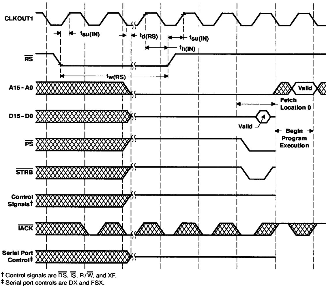
Figure 10. Reset Timing
