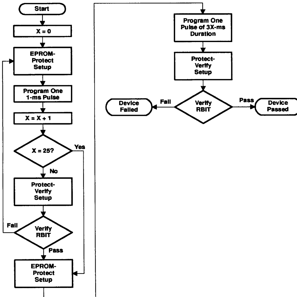
Figure 25. EPROM-Protection Flowchart
