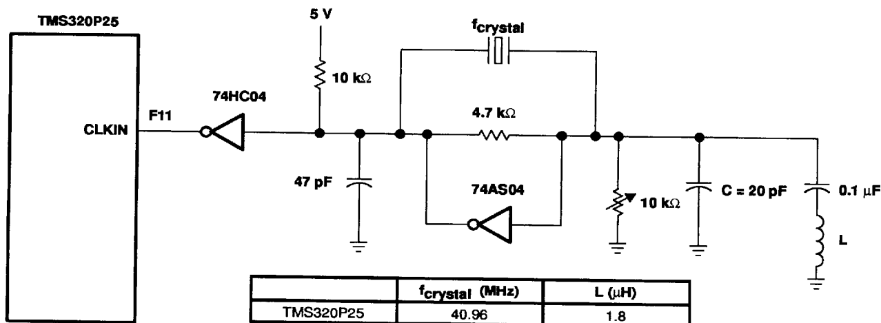
Figure 3. External Clock Option
