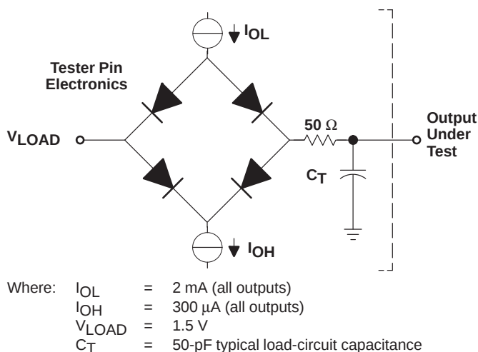
Figure 19. Test Load Circuit
