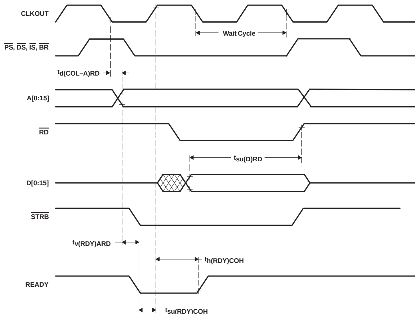
Figure 38. Ready-on-Read Timings
