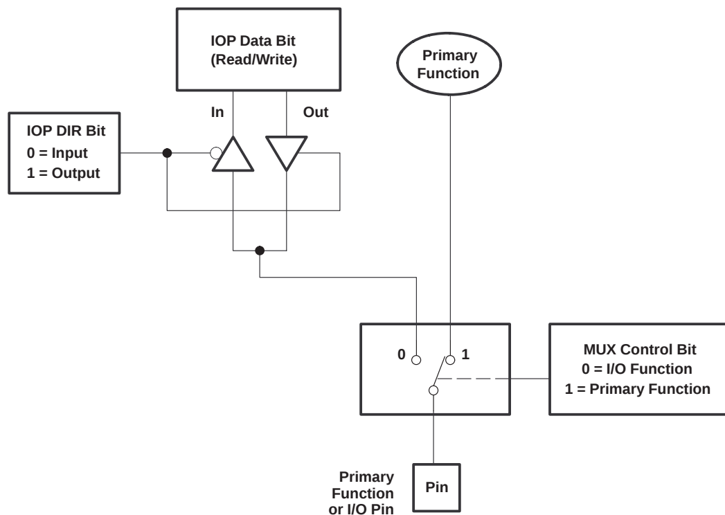
Figure 16. Shared Pin Configuration
