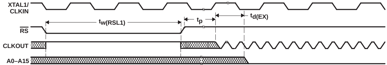
Figure 23. Watchdog Reset Pulse
