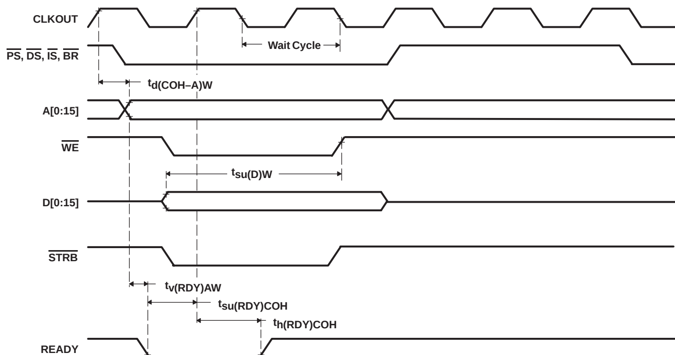
Figure 39. Ready-on-Write Timings
