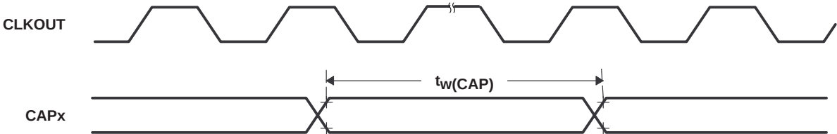
Figure 28. Capture Input and QEP Timing
