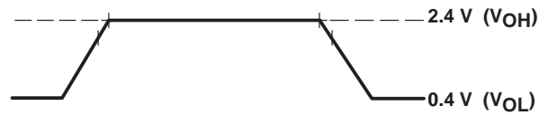
Figure 6–6. Output Levels
