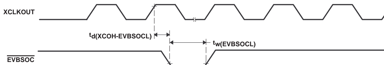
Figure 6–20. \overline{\text{EVBSOC}} Timing
