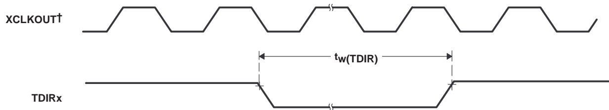
Figure 6–18. TDIRx Timing
