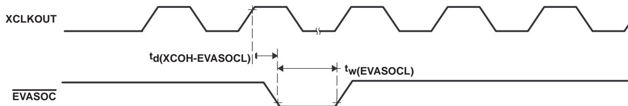
Figure 6–19. \overline{\text{EVASOC}} Timing
