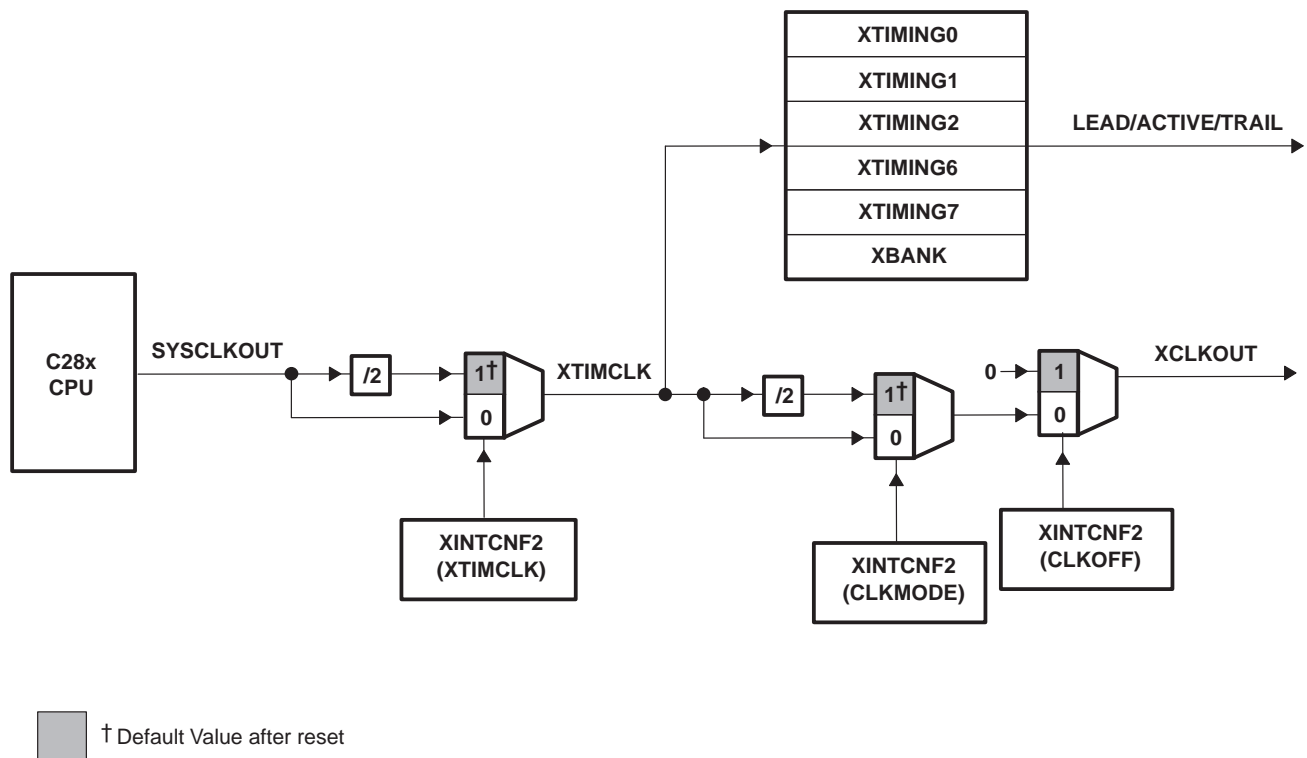
Figure 6–29. Relationship Between XTIMCLK and SYCLKOUT
