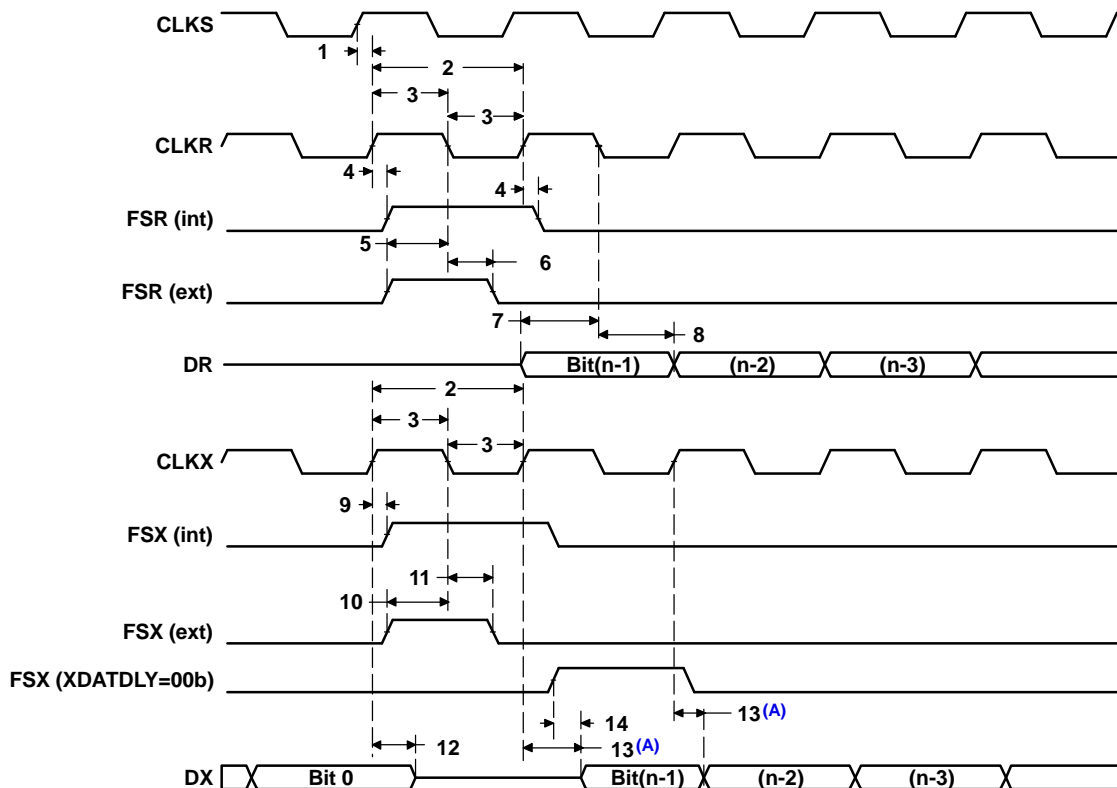
Figure 5-51. McBSP Timing
