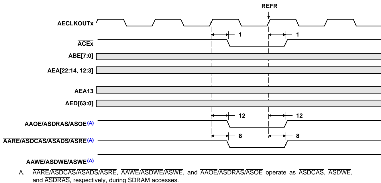
Figure 5-27. SDRAM REFR Command for EMIFA
