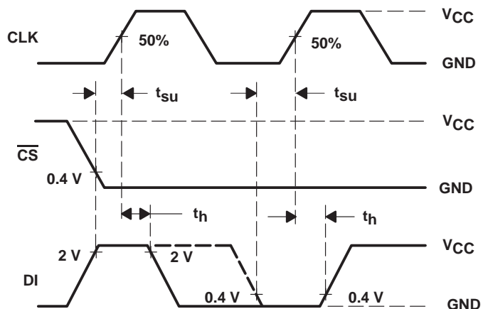
Figure 1. TLV0832 Data-Input Timing
