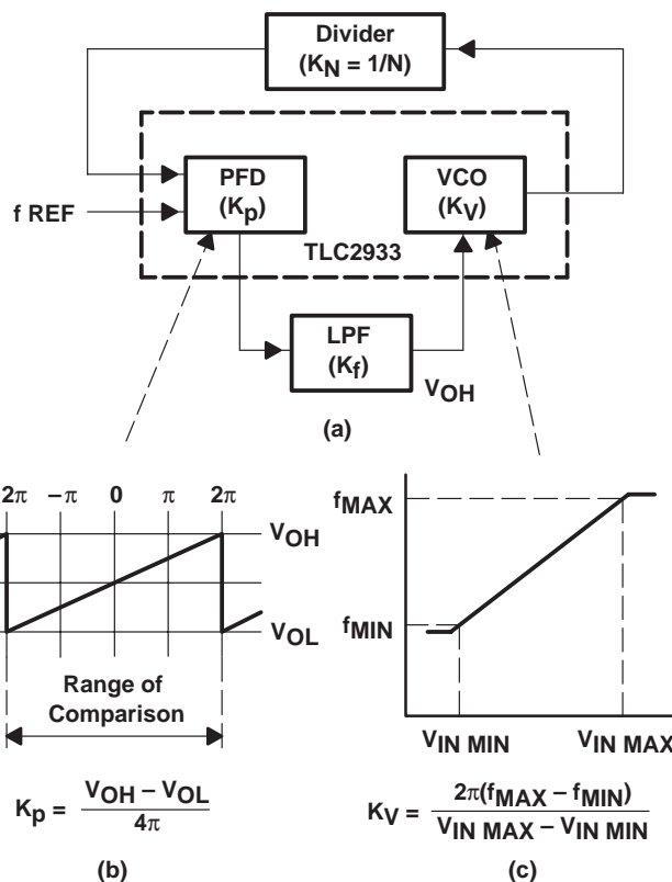
Figure 16. Example of a PLL Block Diagram
