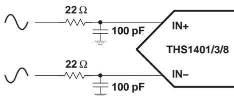
Figure 19. Differential Input
