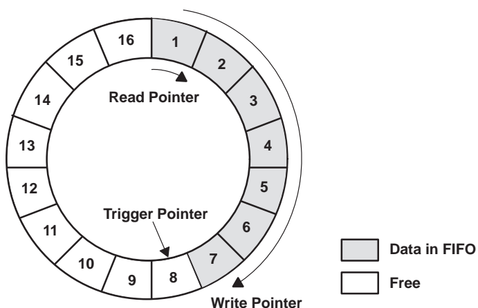
Figure 6. Circular Buffer
