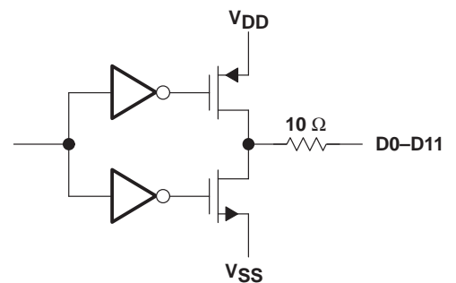
Figure 5. Digital Outputs
