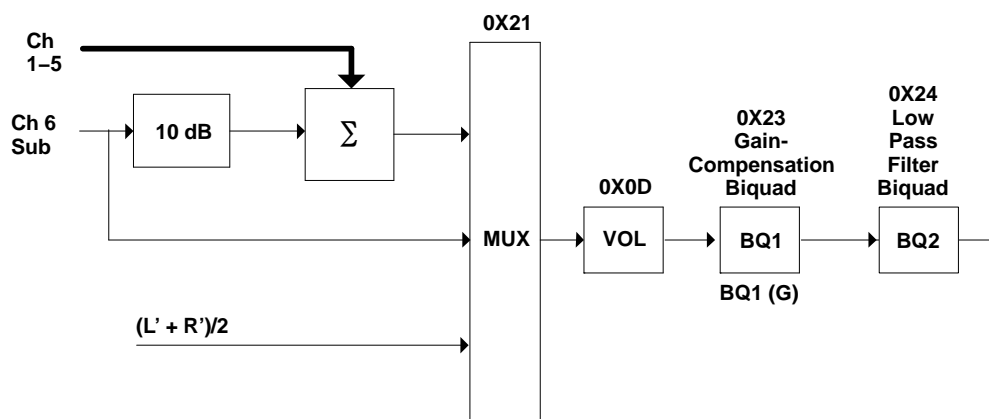
Figure 3. Channel 6 Processing Block Diagram
