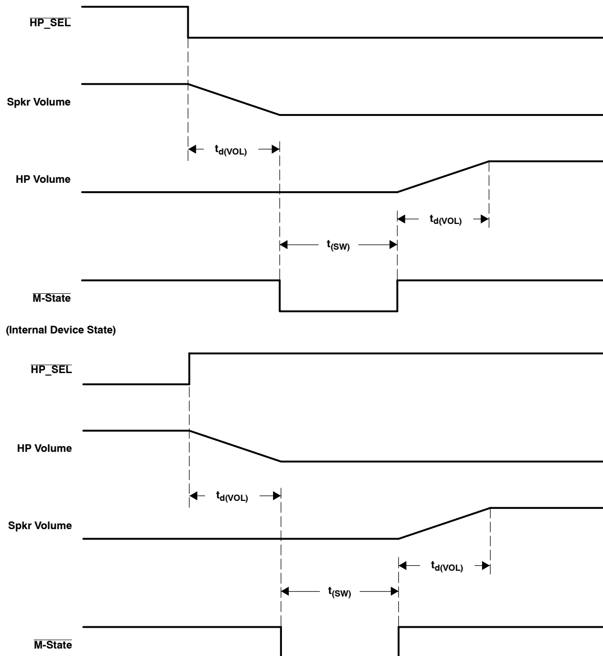
Figure 3–8. HP_SEL Timing
