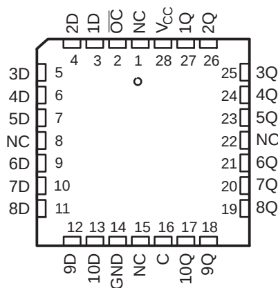
SN54ALS842, SN54AS842 . . . FK PACKAGE SN74ALS842, SN74AS842 . . . FN PACKAGE (TOP VIEW)
