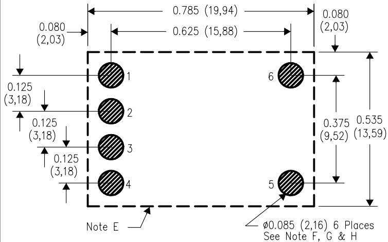
PC LAYOUT
