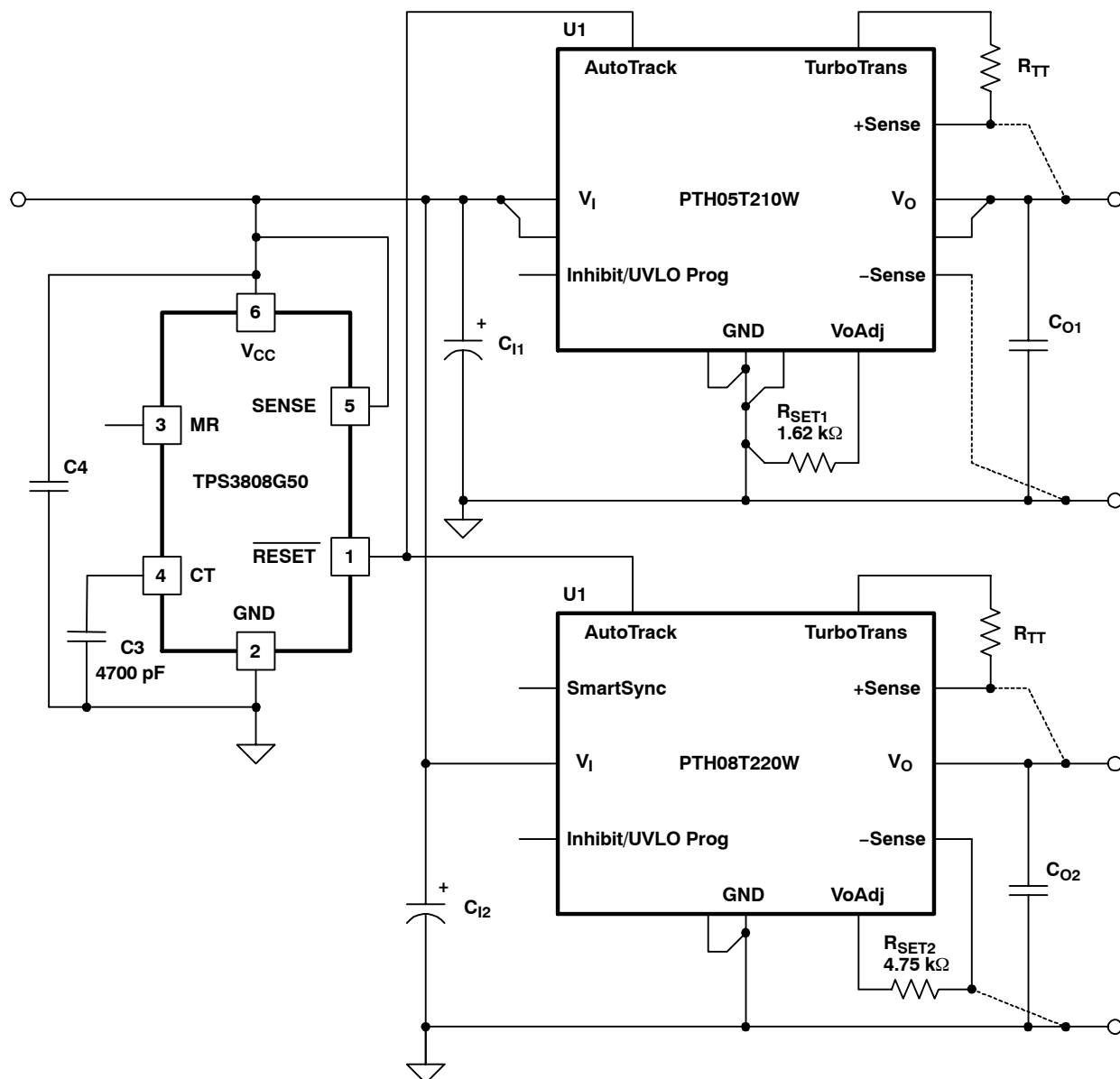
Figure 16. Sequenced Power Up and Power Down Using Auto-Track
