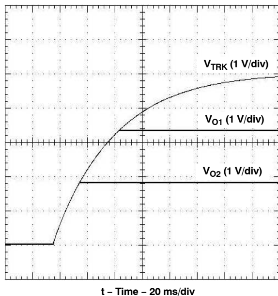
Figure 17. Simultaneous Power Up With Auto-Track Control
