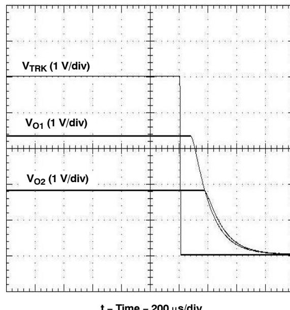
Figure 18. Simultaneous Power Down With Auto-Track Control
