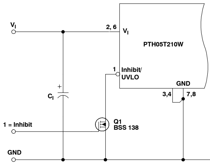
Figure 14. On/Off Inhibit Control Circuit
