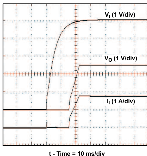
Figure 11. Power-Up Waveform
