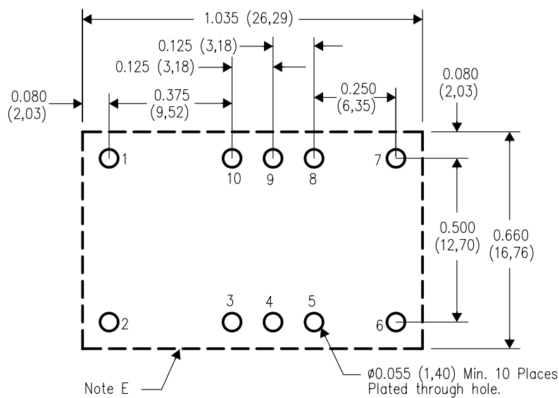
PC LAYOUT
