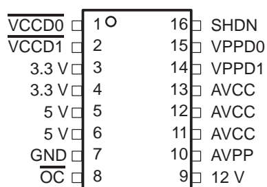
Figure 3–3. TPS2211 Terminal Assignments
