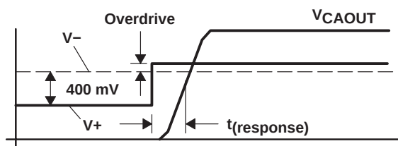
Figure 12. Overdrive Definition
