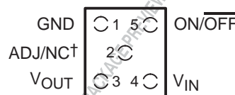
YEQ, YEU, YZQ, OR YZU (WCSP) PACKAGE (TOP VIEW)
