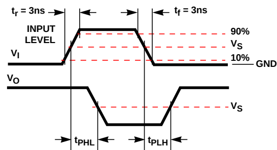
FIGURE 2. PROPAGATION DELAY TIMES
