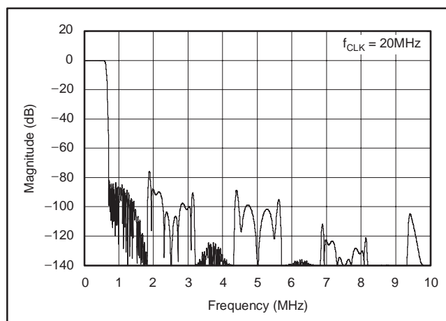
Figure 45. Frequency Response
