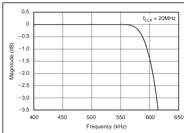
Figure 47. Passband Transition
