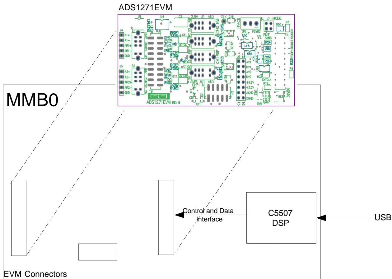
Figure 2. ADS1271EVM-PDK Block Diagram
