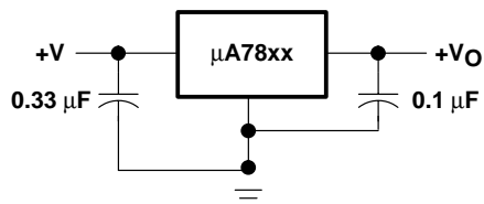
Figure 1. Fixed-Output Regulator
