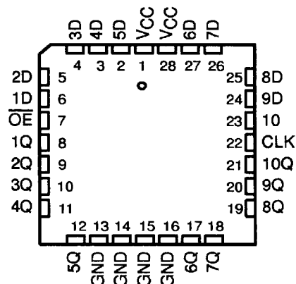
54ACT11821 ... FK PACKAGE (TOP VIEW)
