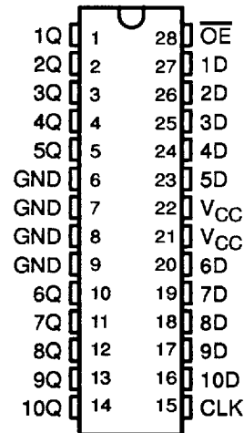
54ACT11821 ... JT PACKAGE 74ACT11821 ... DW PACKAGE (TOP VIEW)
