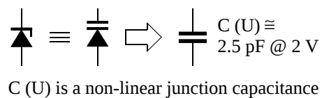
Figure 11. ESD-protection diodes
