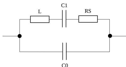
Figure 23. Equivalent crystal circuit
