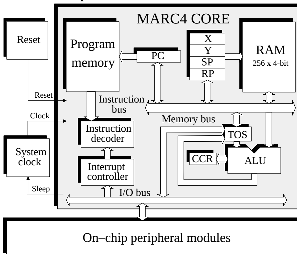
Figure 4. MARC4 core
