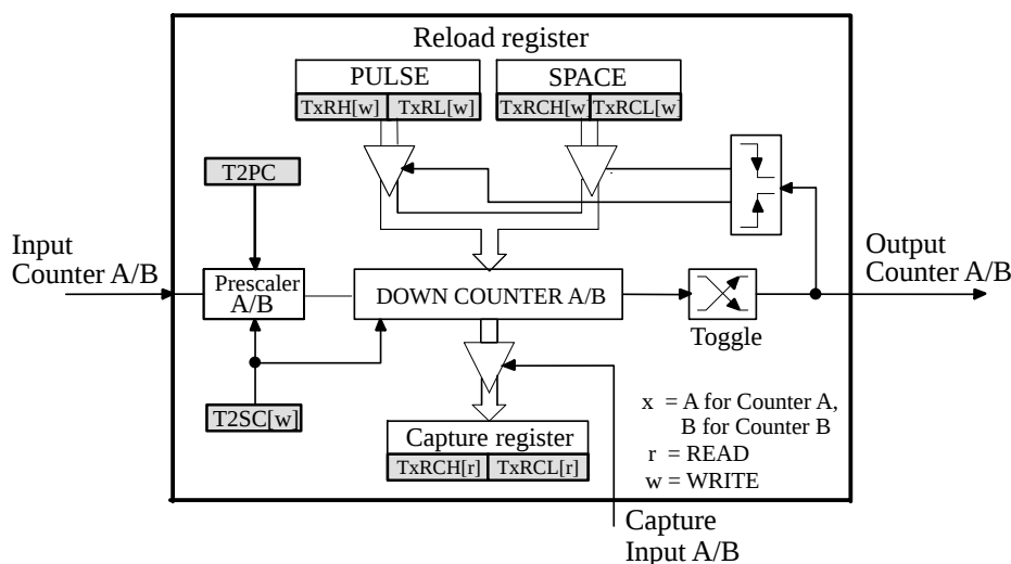
Figure 18. Counter A/B
