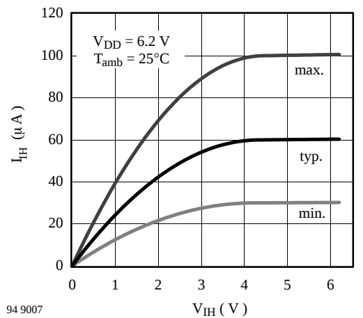
Figure 40. Input HIGH current vs. input HIGH voltage
