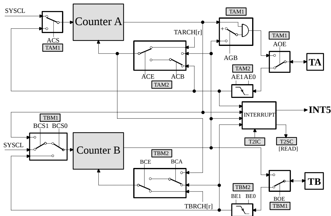
Figure 17. Timer 2
