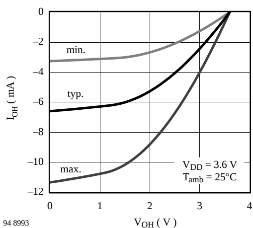
Figure 30. Output HIGH current vs. output HIGH voltage
