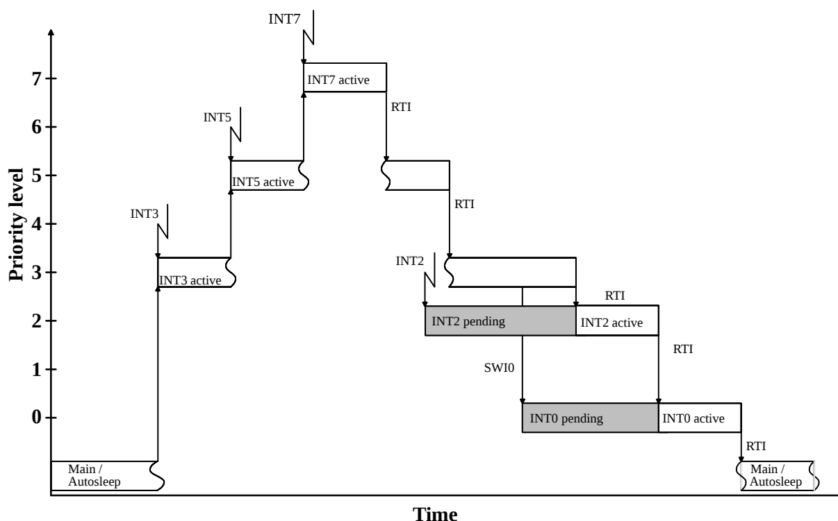
Figure 9. Interrupt handling
