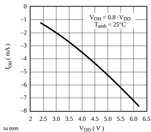
Figure 27. Output HIGH current vs. supply voltage
