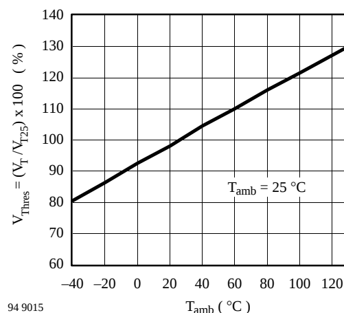
Figure 48. Threshold temperature drift
