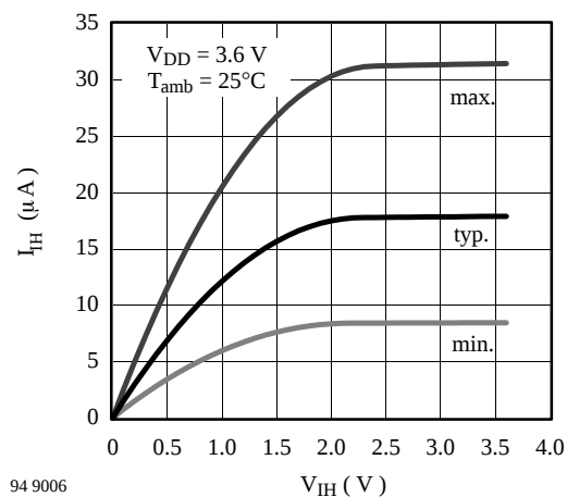
Figure 39. Input HIGH current vs. input HIGH voltage
