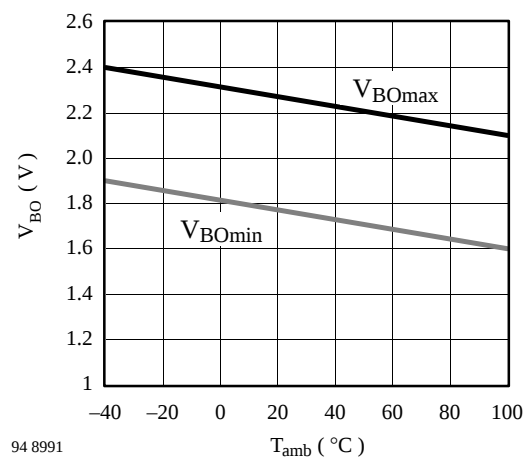
Figure 24. Brown-out voltage vs. ambient temperature
