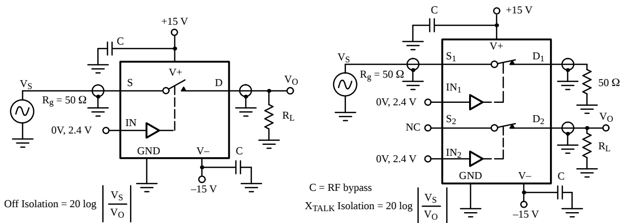
Figure 4. Off Isolation
