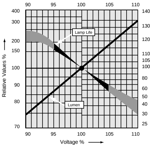
Life/Lumen-Volt Characteristic
