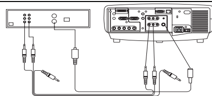
connect S-video and video cables
