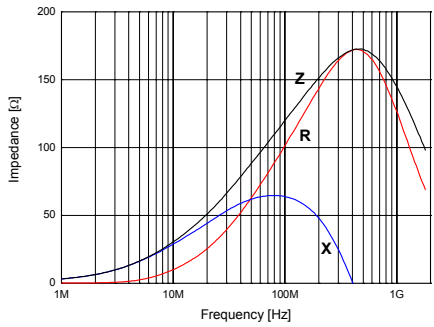
SHB-1T1608-121J
