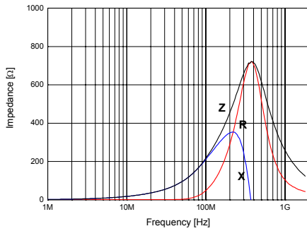
SHB-1S1608-221J
