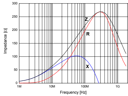
SHB-1T1608-221J
