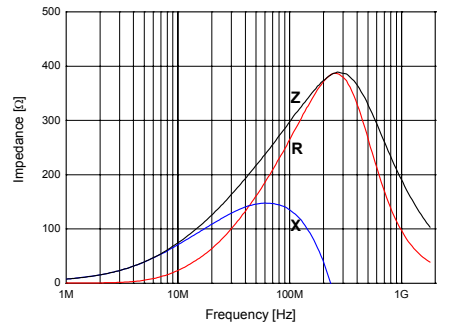
SHB-1T1608-301J
