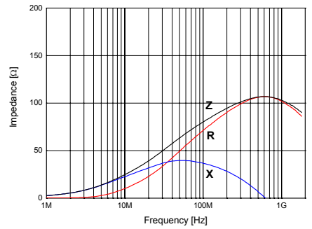
SHB-1T1608-800J
