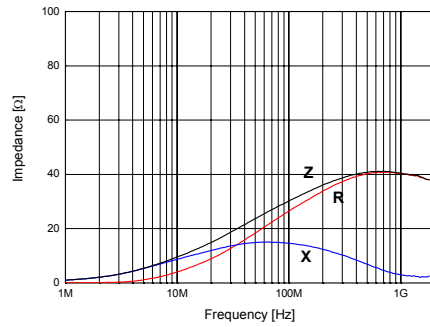
SHB-1T1608-300J
