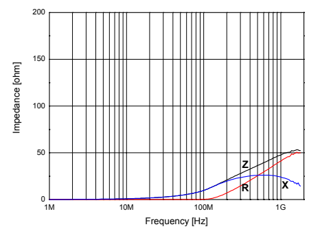
SHB-1S1608-100J
