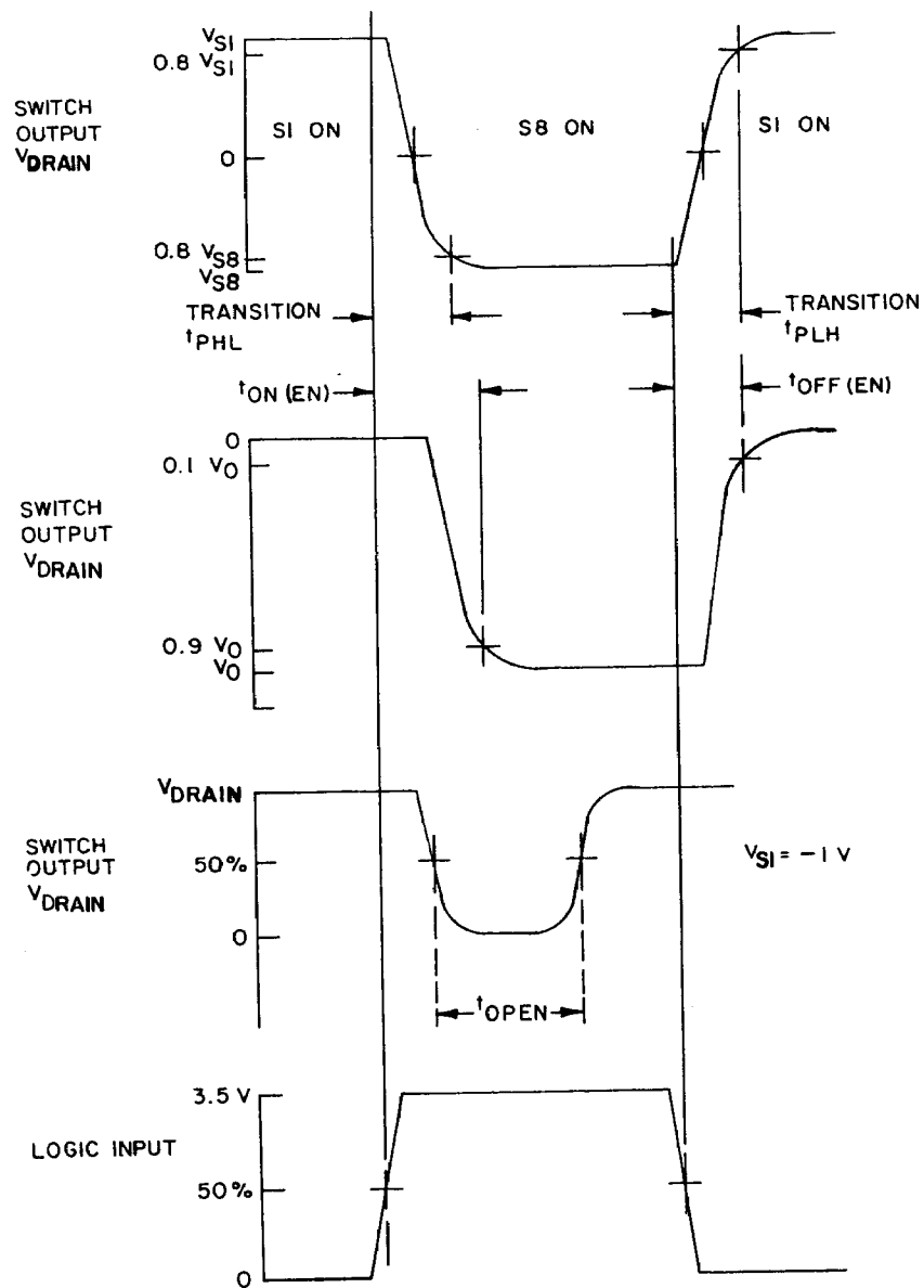
FIGURE 5. Switching time waveforms.
