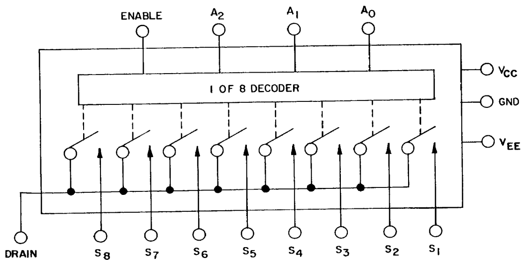
FIGURE 2. Logic diagram.
