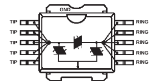
PowerSO-10™ TLPxxM
