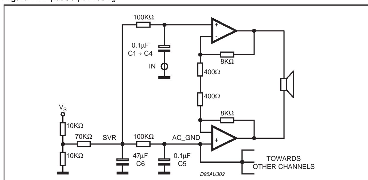
Figure 11: Input/Output Biasing.
