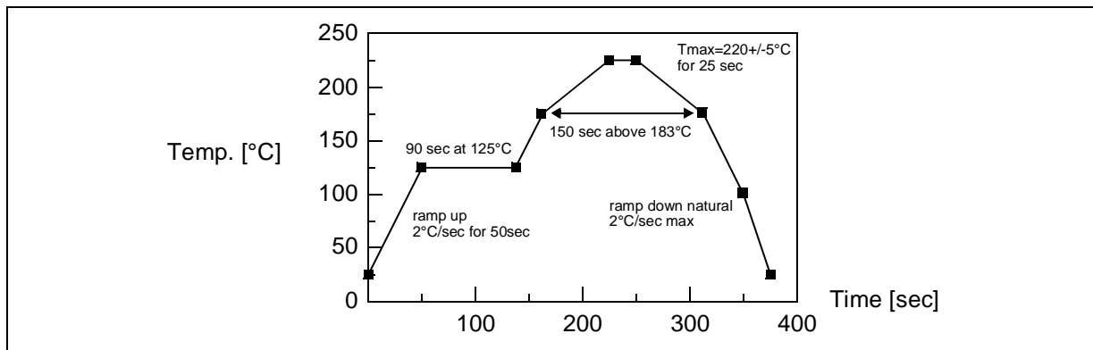
Figure 109. Recommended Reflow Oven Profile (MID JEDEC)
