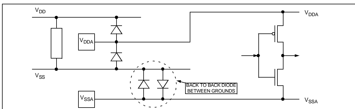
Figure 86. Multisupply Configuration
