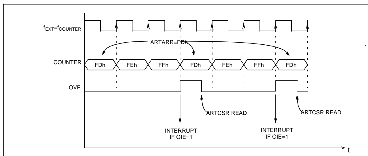
Figure 44. External Event Detector Example (3 counts)
