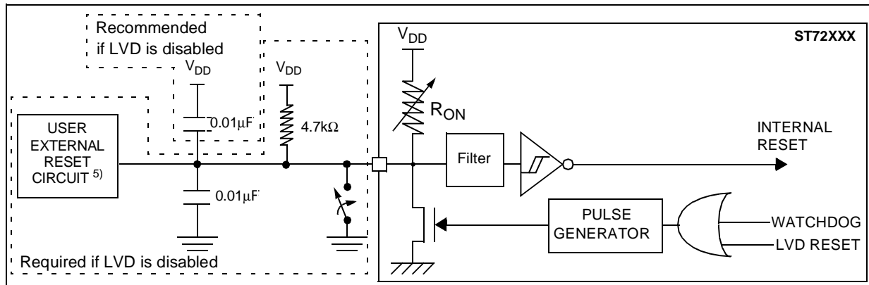
Figure 99. Typical Application with RESET pin 6)7)8)
