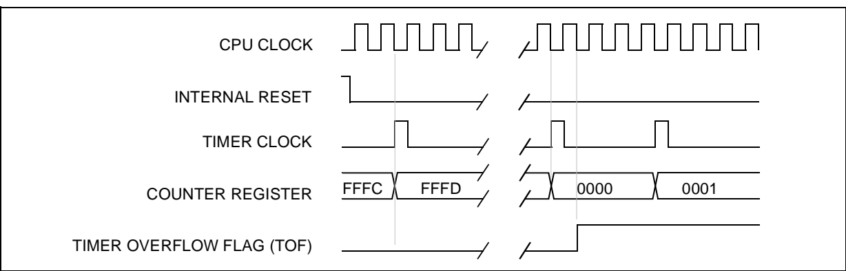
Figure 38. Counter Timing Diagram, internal clock divided by 4
