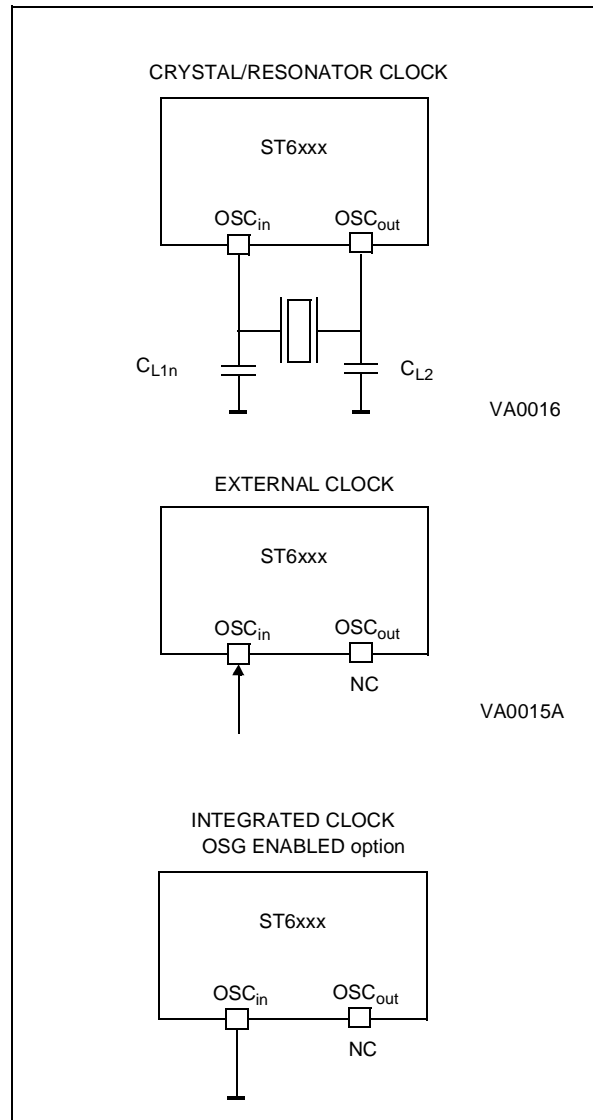
Figure 9. Oscillator Configurations
