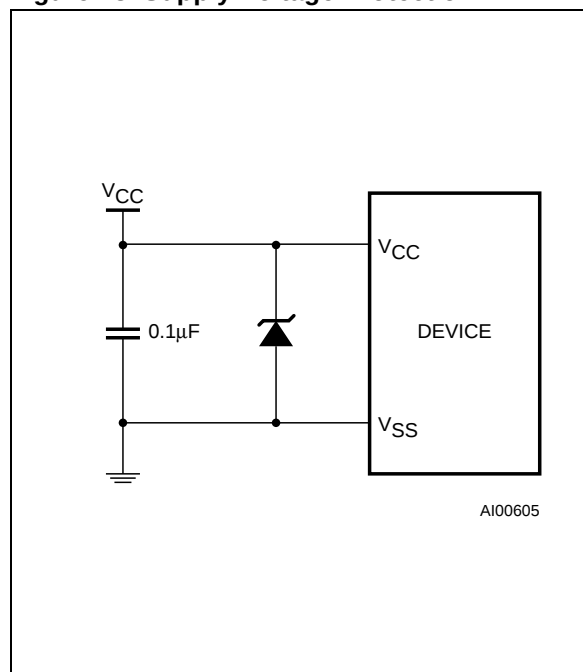
Figure 13. Supply Voltage Protection
