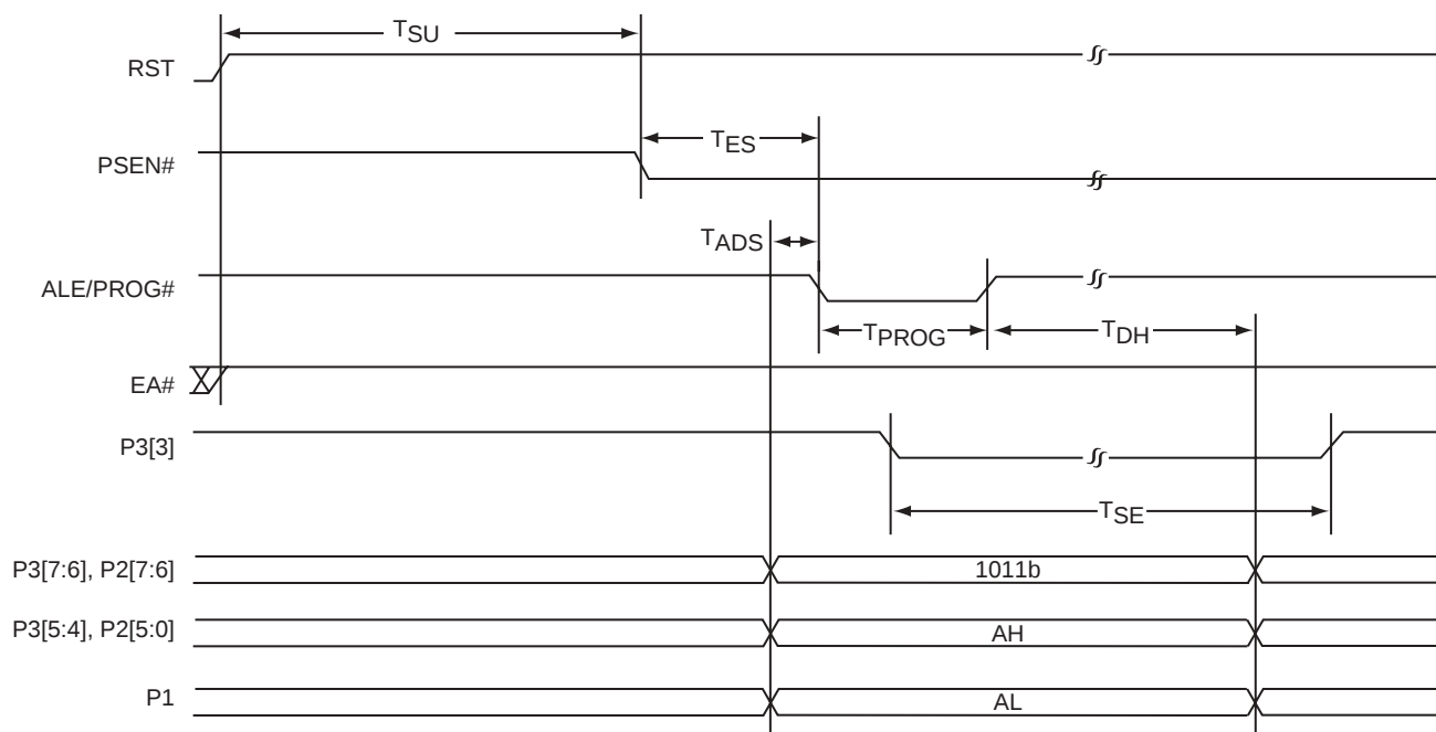
FIGURE 14-19: SECTOR-ERASE
